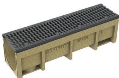
SF-200 channel with slotted ductile-iron grating cl. F900'
